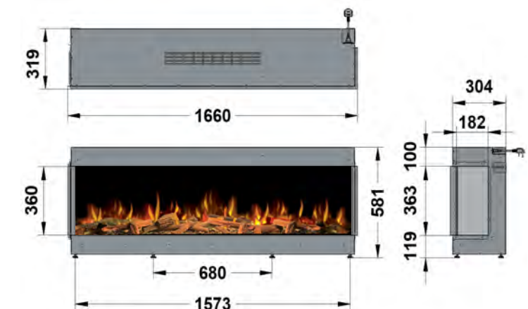
1650 - RIGHT CORNER
